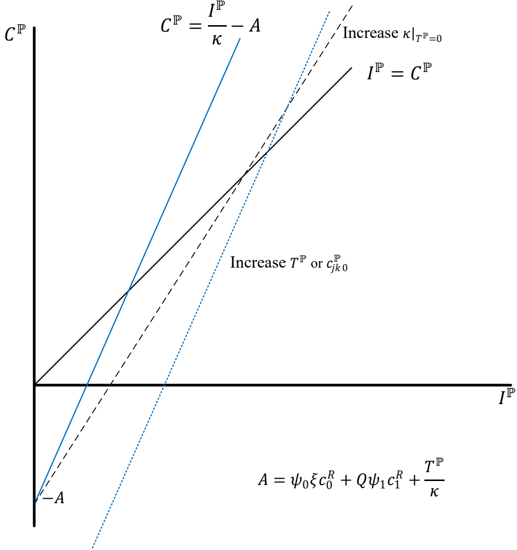
Figure 2. Graphical proof of Proposition 1.
