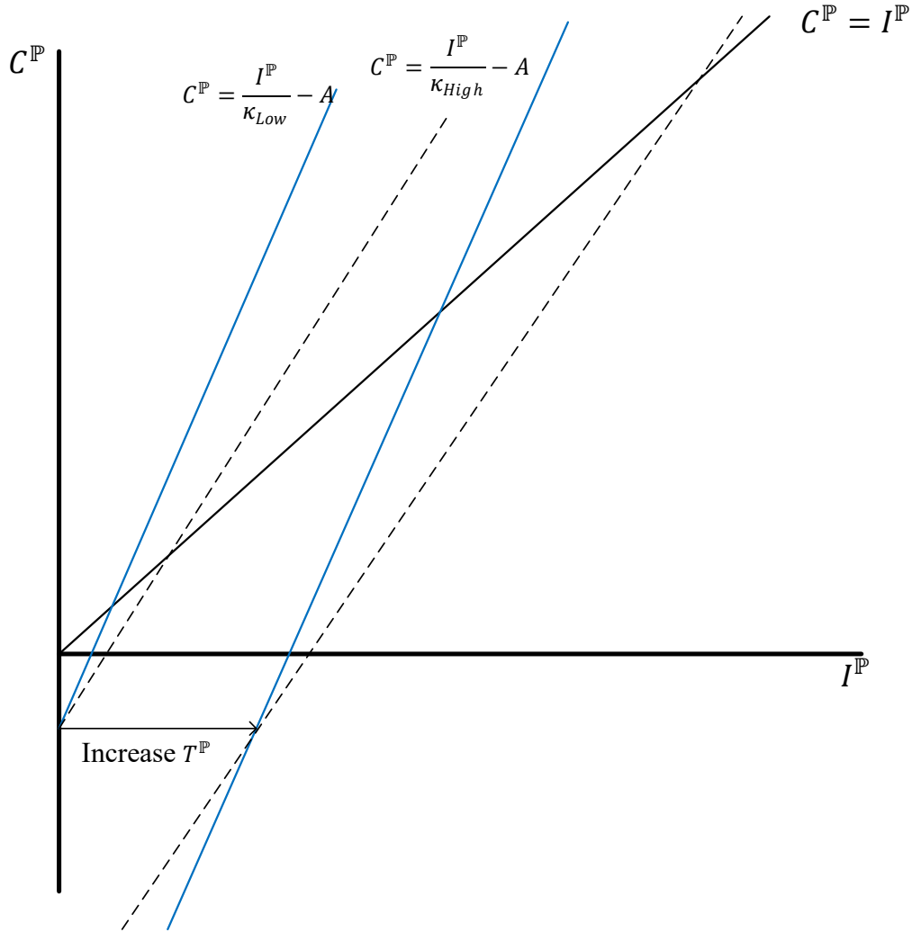
Figure 3. Higher Income Share of the Poor Implies higher Fiscal Multipliers.
